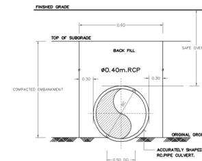
PIPE BEDDING FOR NON - TRAFFIC
