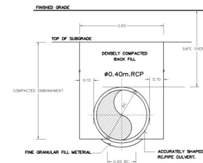
TYPICAL INSTALLATION OF TRENCH CONDUIT
