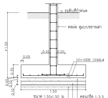
F3 1: 25
