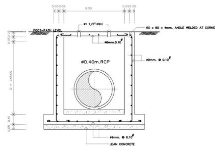
SECTION 3 SCALE 1:10
