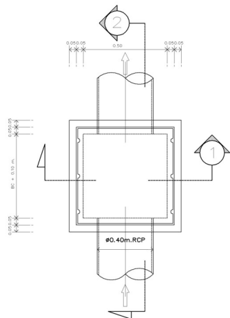
PLAN MANHOLE SCALE 1:10
