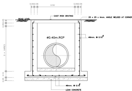
SECTION 1 SCALE 1:10
