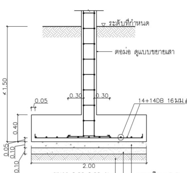
F5 1: 25
