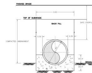
PIPE BEDDING FOR TRAFFIC
