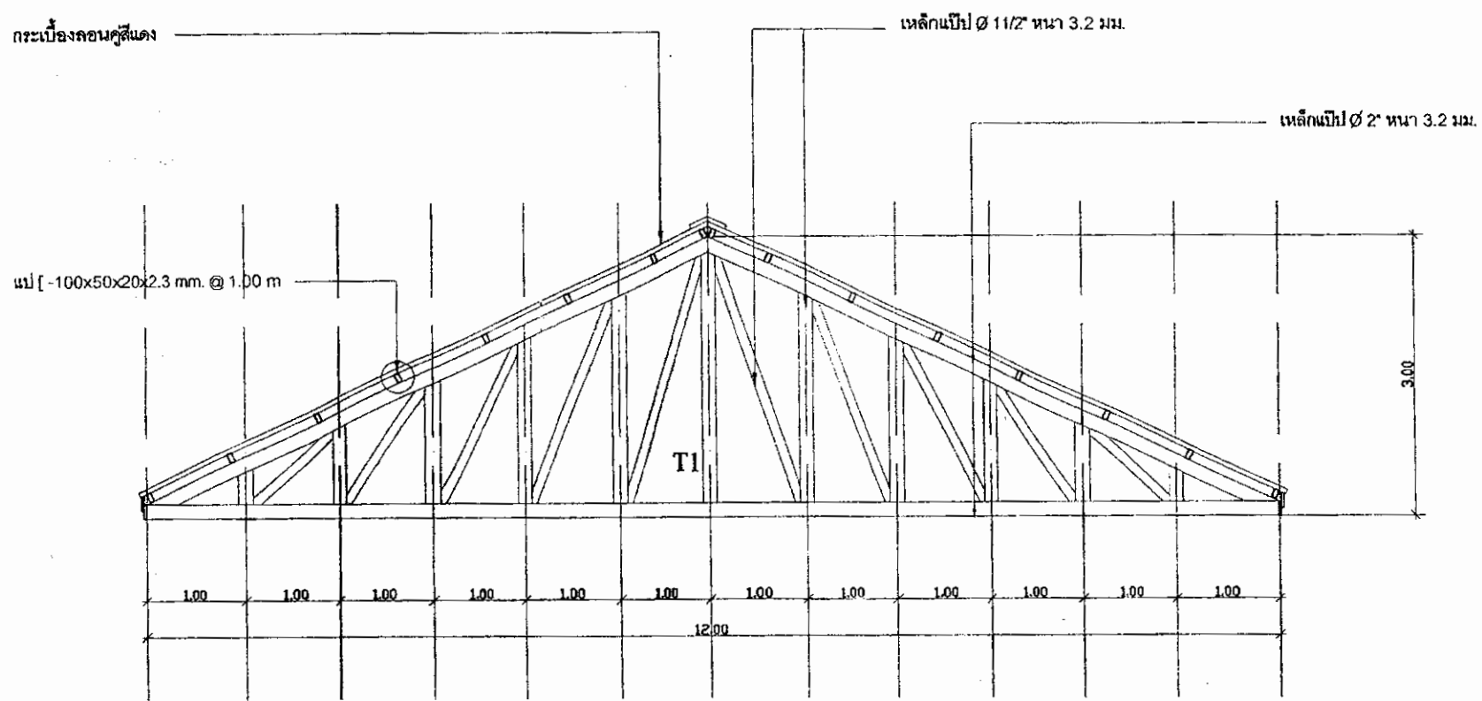
TRUSS 1
