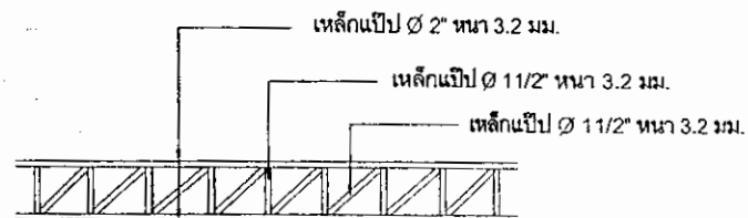
TRUSS 3
