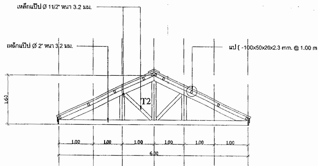
TRUSS 2
