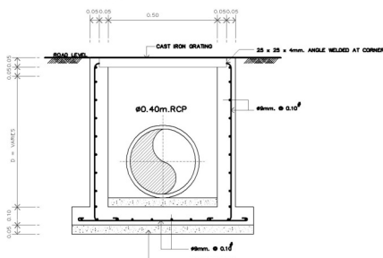
SECTION 1 SCALE 1:10
