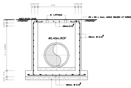
SECTION 3 SCALE 1:10
