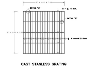
CAST STAINLESS GRATING
