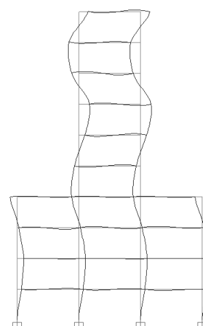
Mode 5 T_5 = 0.132 \text{ sec}
