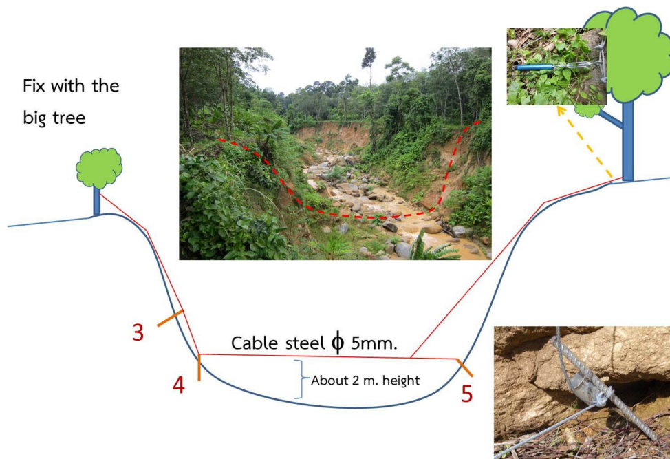
3, 4 and 5 main cable fix with pin.
