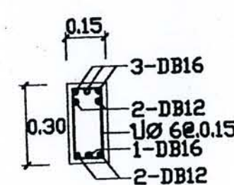
SECTION 1-1
