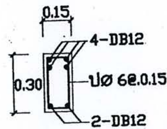
SECTION 1-1
