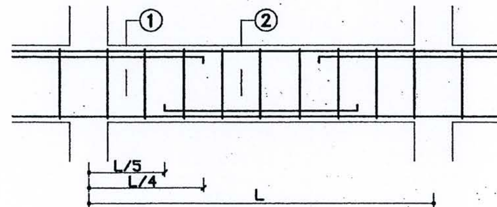
LONG SECTION
