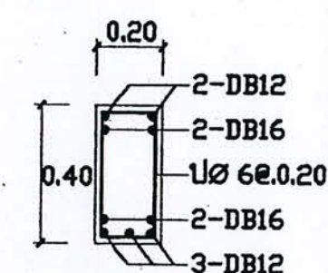
SECTION 2-2
