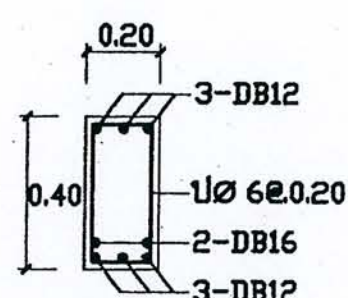
SECTION 2-2
