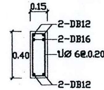
SECTION 1-1
