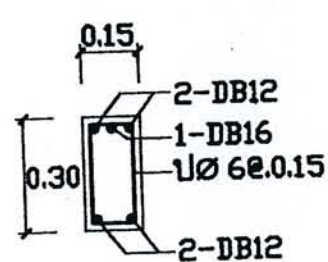
SECTION 1-1
