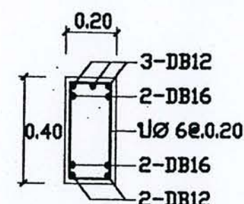
SECTION 1-1
