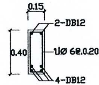
SECTION 2-2
