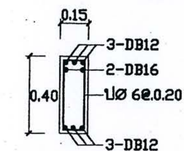
SECTION 1-1
