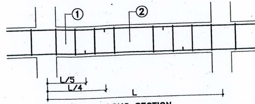
LONG SECTION
