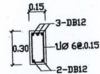
SECTION 1-1
