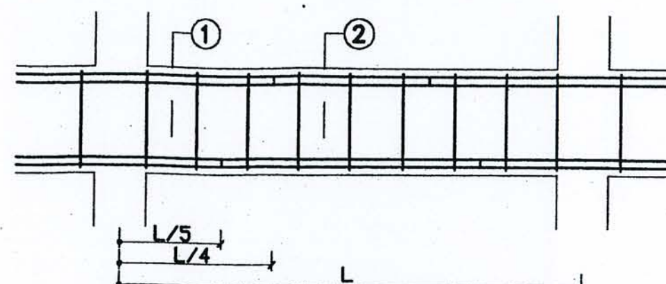
LONG SECTION
