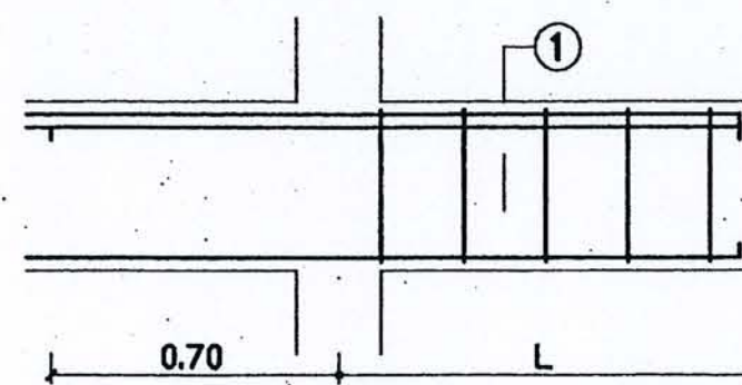
LONG SECTION
