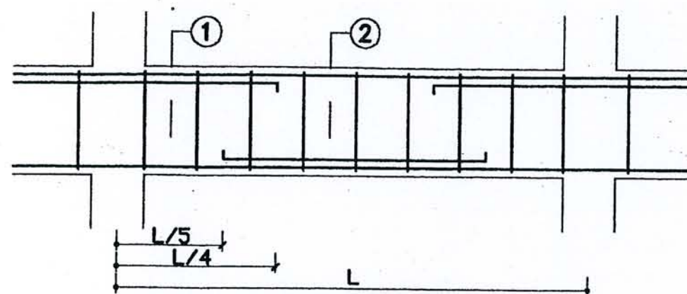
LONG SECTION
