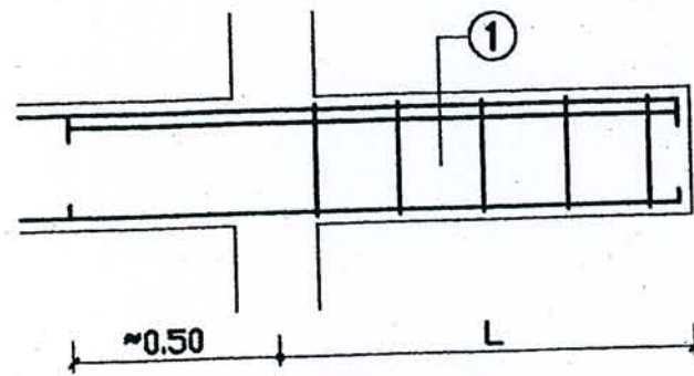
LONG SECTION
