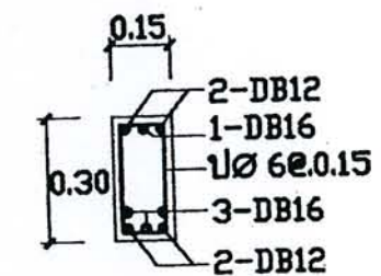
SECTION 2-2
