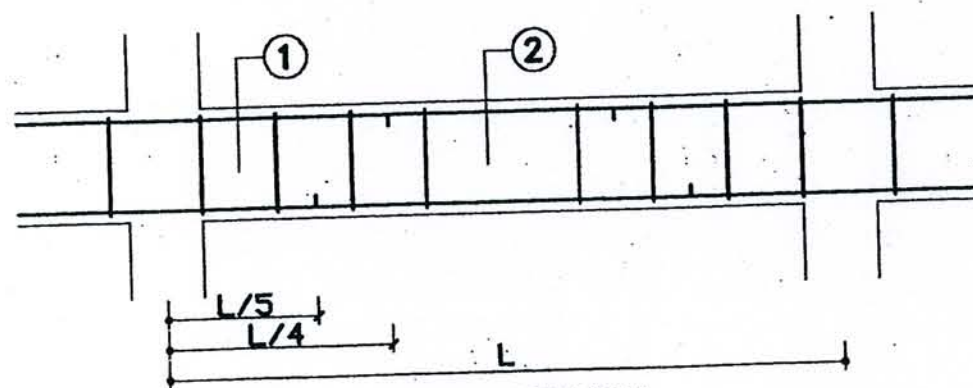
LONG SECTION
