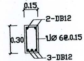
SECTION 2-2
