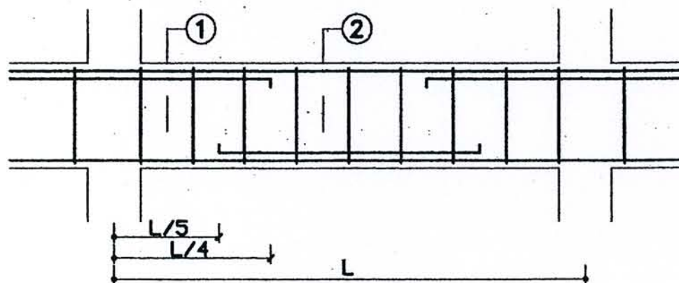
LONG SECTION
