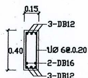
SECTION 2-2
