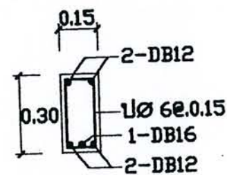
SECTION 2-2
