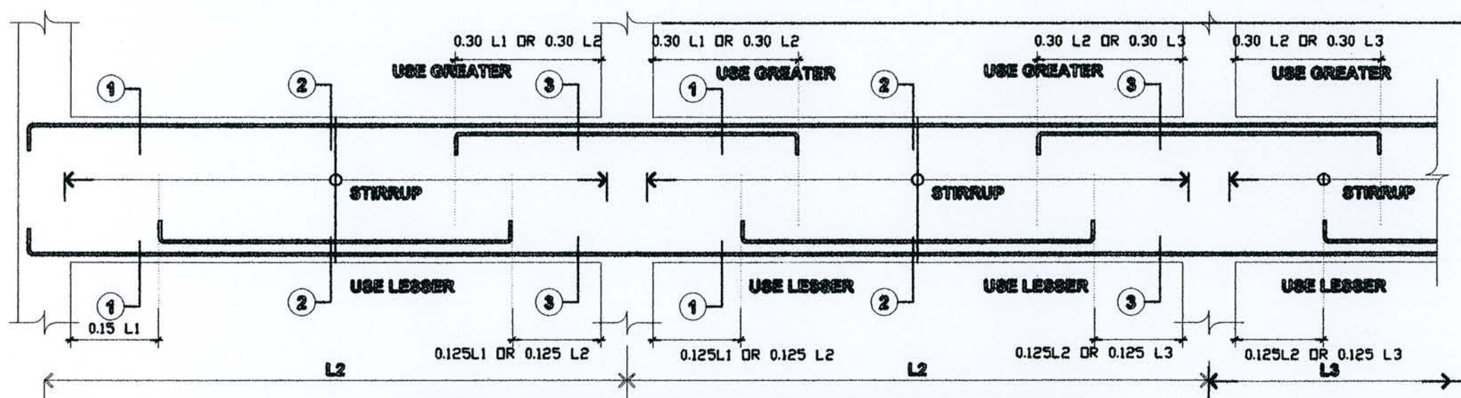
TYPICAL ARRANGEMENT OF CONTINUOUS BEAM
