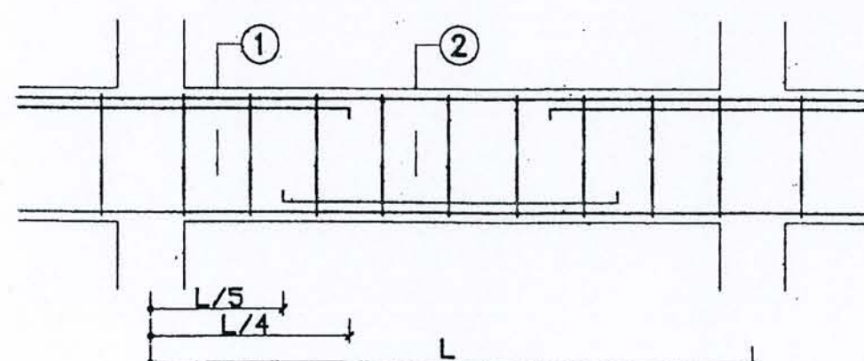
LONG SECTION
