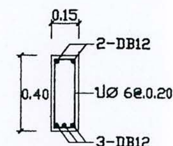
SECTION 2-2
