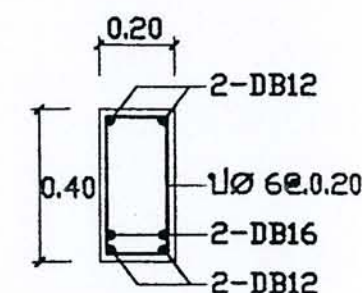
SECTION 2-2
