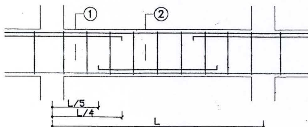
LONG SECTION
