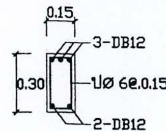
SECTION 1-1
