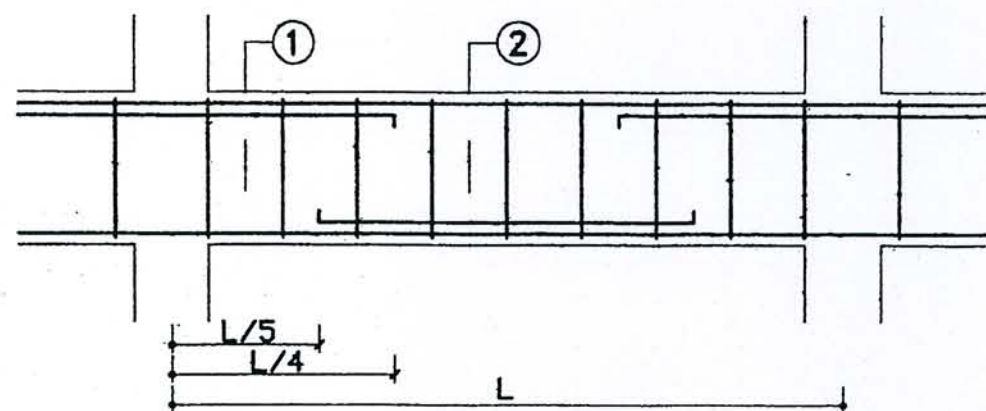
LONG SECTION
