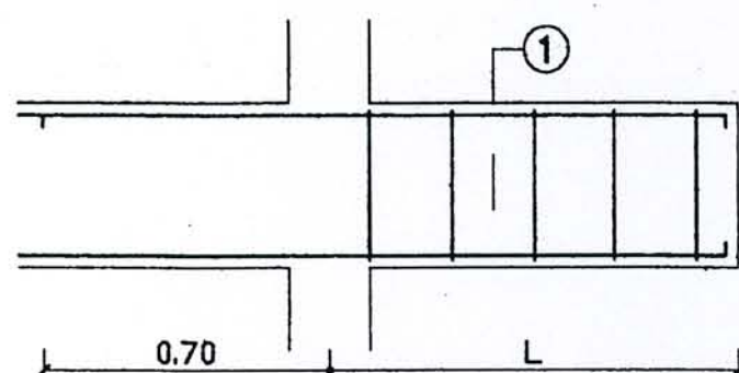
LONG SECTION
