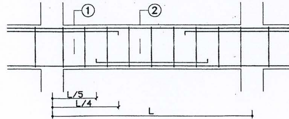
LONG SECTION
