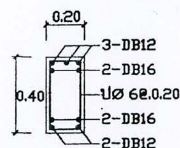
SECTION 1-1
