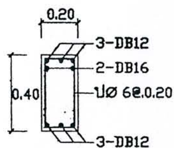
SECTION 1-1
