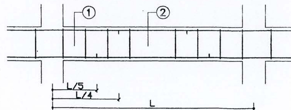
LONG SECTION
