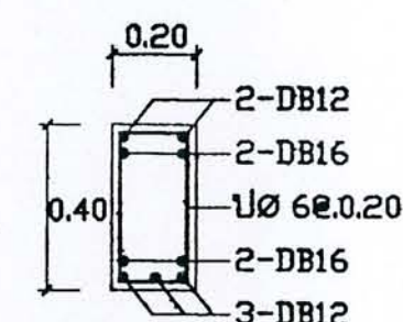
SECTION 2-2
