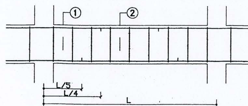
LONG SECTION
