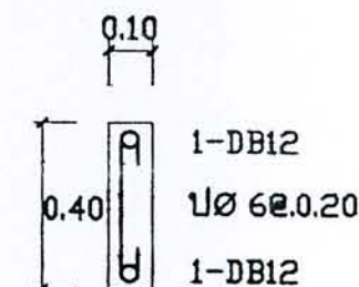
SECTION 2-2
