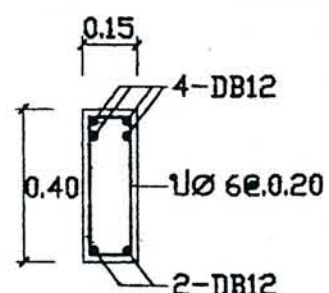
SECTION 1-1
