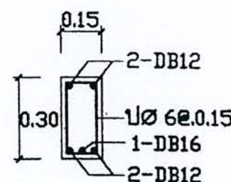
SECTION 2-2
