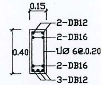
SECTION 2-2
