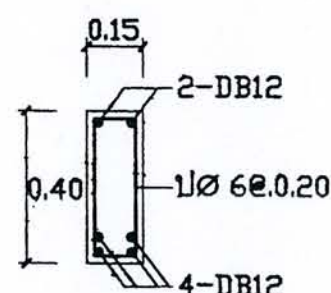
SECTION 2-2
