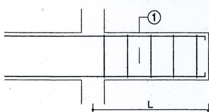
LONG SECTION
