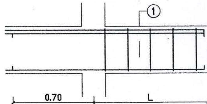
LONG SECTION
