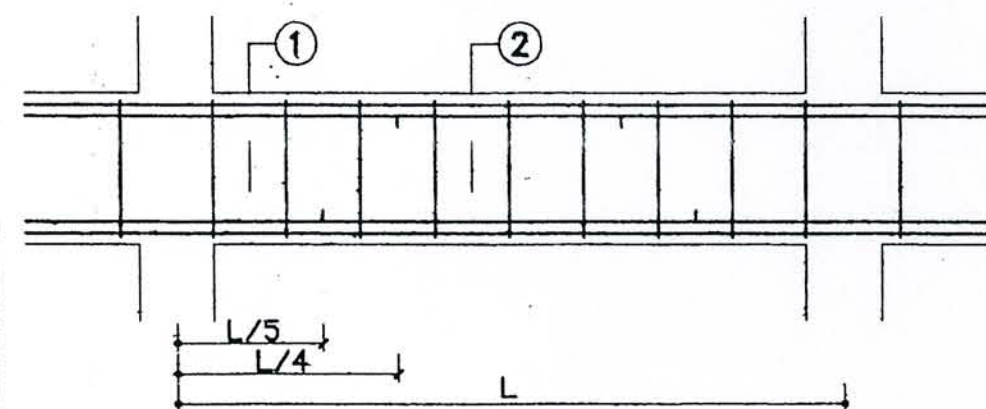
LONG SECTION
