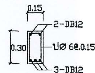
SECTION 2-2
