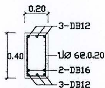
SECTION 2-2
