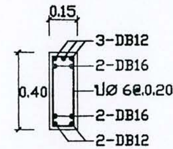
SECTION 1-1
