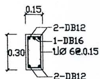
SECTION 1-1
