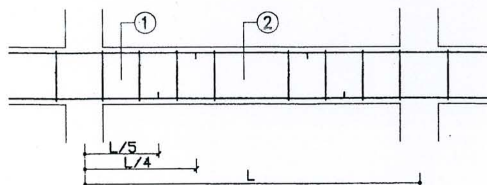
LONG SECTION
