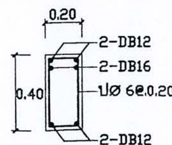
SECTION 1-1
